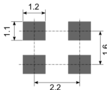
< Pad Pattern >
