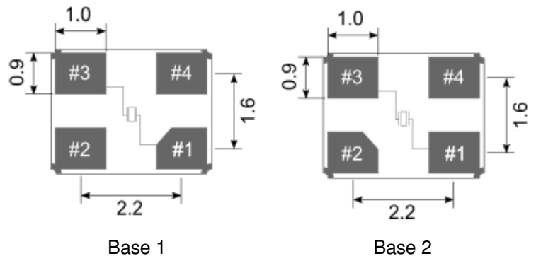
< Pad Pattern >
